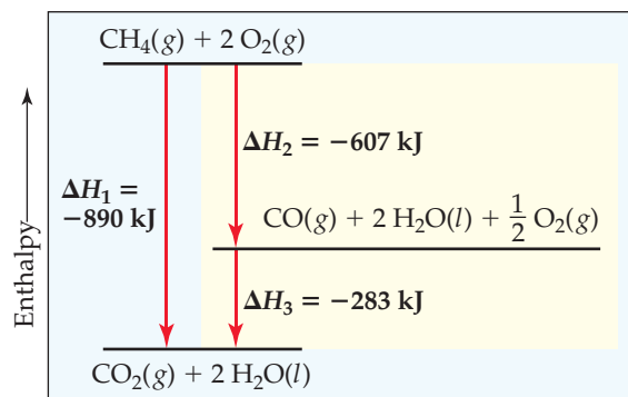
▲ Figure 5.21 Enthalpy diagram illustrating Hess's law. The net reaction is the same as in Figure 5.20, but here we imagine different reactions in our two-step version. As long as we can write a series of equations that add up to the equation we need, and as long as we know a value for \Delta H for all intermediate reactions, we can calculate the overall \Delta H .
