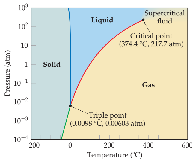
▲ Figure 11.28 Phase diagram of H 2 O. Note that a linear scale is used to represent temperature and a logarithmic scale to represent pressure.
