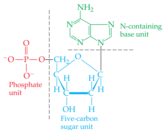
▲ Figure 24.27 A nucleotide. Structure of deoxyadenylic acid, the nucleotide formed from phosphoric acid, the sugar deoxyribose, and the organic base adenine.
