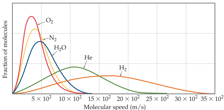
▲ Figure 10.14 The effect of molar mass on molecular speed at 25 °C.
