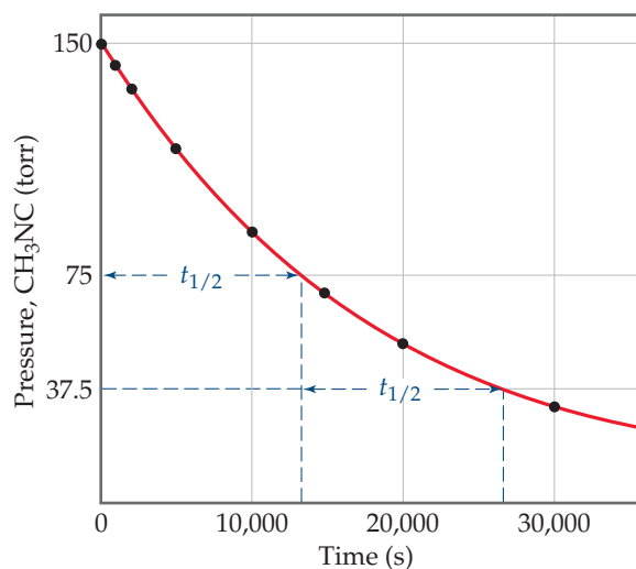
▲ Figure 14.11 Kinetic data for the rearrangement of methyl isonitrile to acetonitrile at 199^\circ\text{C} , showing the half-life of the reaction.
