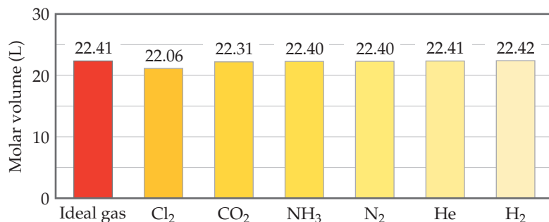
▲ Figure 10.10 Comparison of molar volumes at STP.
