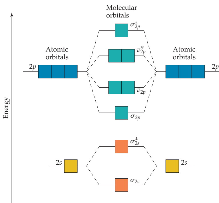
▲ Figure 9.41 Energy-level diagram for MOs of period 2 homonuclear diatomic molecules. The diagram assumes no interaction between the 2s atomic orbital on one atom and the 2p atomic orbitals on the other atom, and experiment shows that it fits only for O 2 , F 2 , and Ne 2 .
