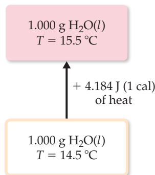
▲ Figure 5.16 Specific heat of water.
