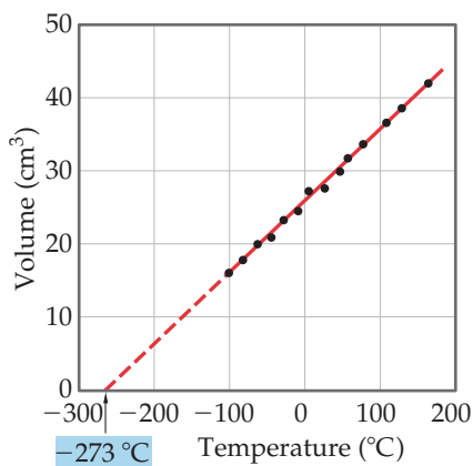
▲ Figure 10.8 Charles’s Law. For a fixed quantity of gas at constant pressure, the volume of the gas is proportional to its temperature.
