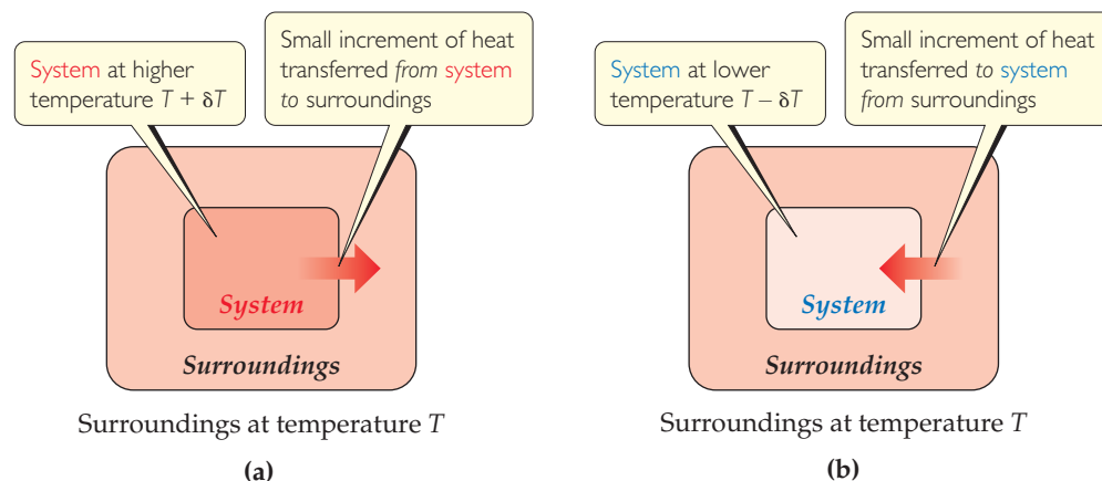
▲ Figure 19.4 Reversible flow of heat. Heat can flow reversibly between a system and its surroundings only if the two have an infinitesimally small difference in temperature \delta T . (a) Increasing the temperature of the system by \delta T causes heat to flow from the hotter system to the colder surroundings. (b) Decreasing the temperature of the system by \delta T causes heat to flow from the hotter surroundings to the colder system.
