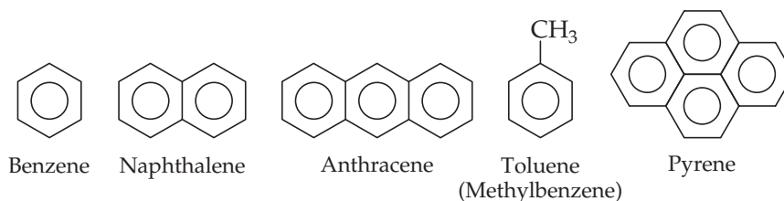
▲ Figure 24.10 Line formulas and common names of several aromatic compounds.
