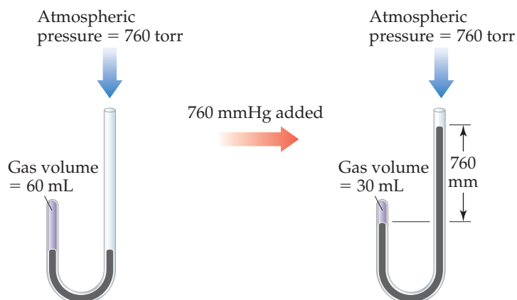
▲ Figure 10.5 Boyle's experiment relating pressure and volume for a gas.
