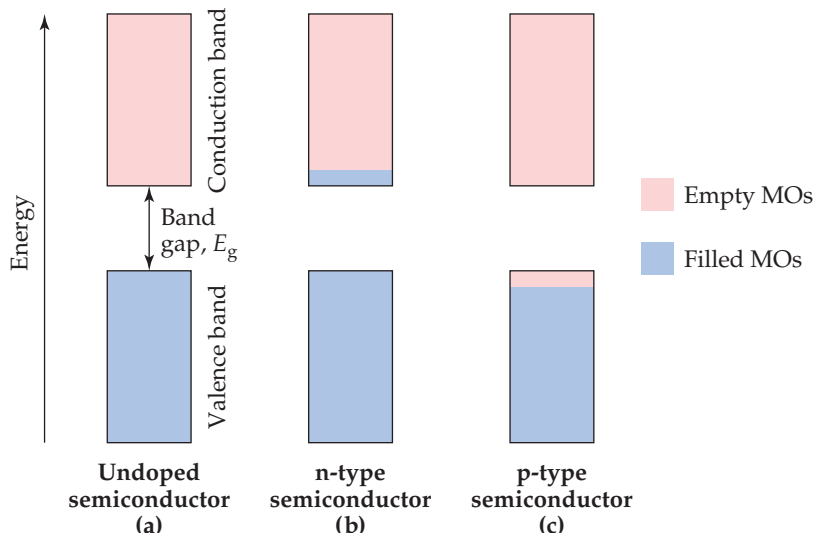
▲ Figure 12.31 The addition of small amounts of impurities (doping) to a semiconductor changes the electronic properties of the material.
