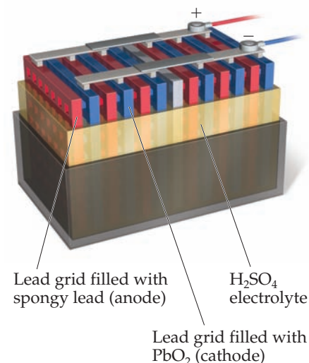
► Figure 20.19 A 12-V automotive lead–acid battery. Each anode/cathode pair in this schematic cutaway produces a voltage of about 2 V. Six pairs of electrodes are connected in series, producing 12 V.
