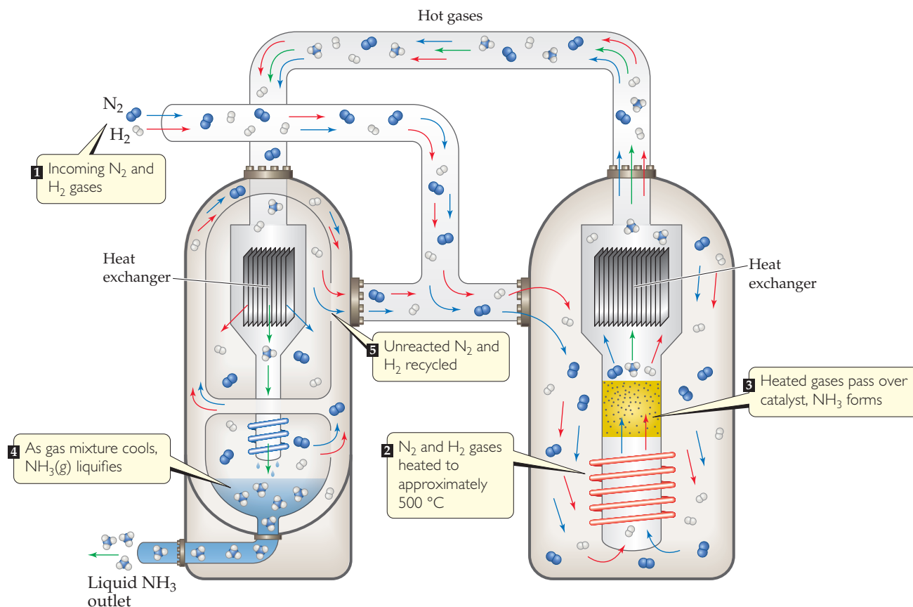
▲ Figure 15.11 Diagram of the industrial production of ammonia. Incoming \text{N}_2(\text{g}) and \text{H}_2(\text{g}) are heated to approximately 500\text{ }^\circ\text{C} and passed over a catalyst. When the resultant \text{N}_2 , \text{H}_2 , and \text{NH}_3 mixture is cooled, the \text{NH}_3(\text{g}) liquefies and is removed from the mixture, shifting the reaction to produce more \text{NH}_3 .
