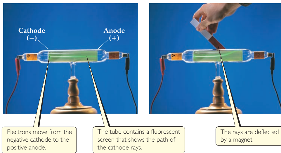
▲ Figure 2.3 Cathode-ray tube.
