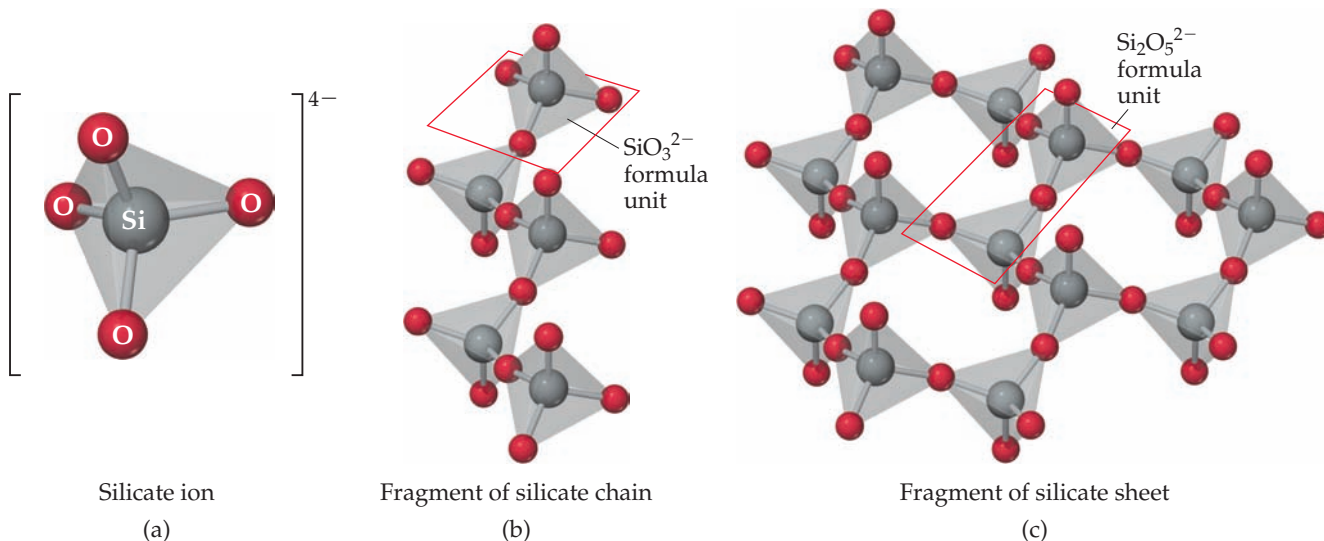
▲ Figure 22.33 Silicate chains and sheets.
