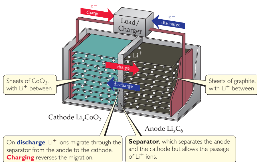
▲ Figure 7.9 Schematic of a lithium-ion battery.
