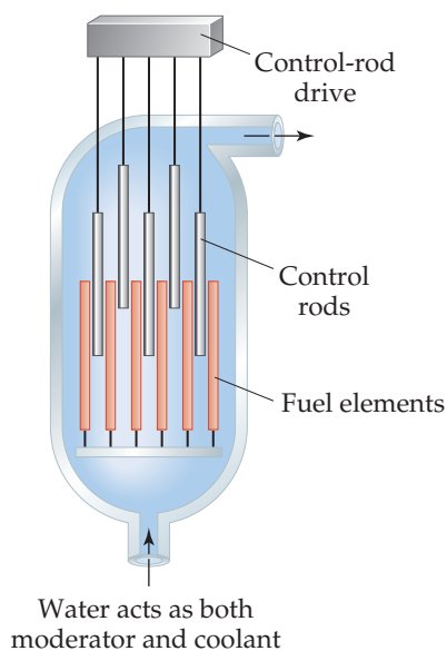
▲ Figure 21.18 Schematic diagram of a pressurized water reactor core.
