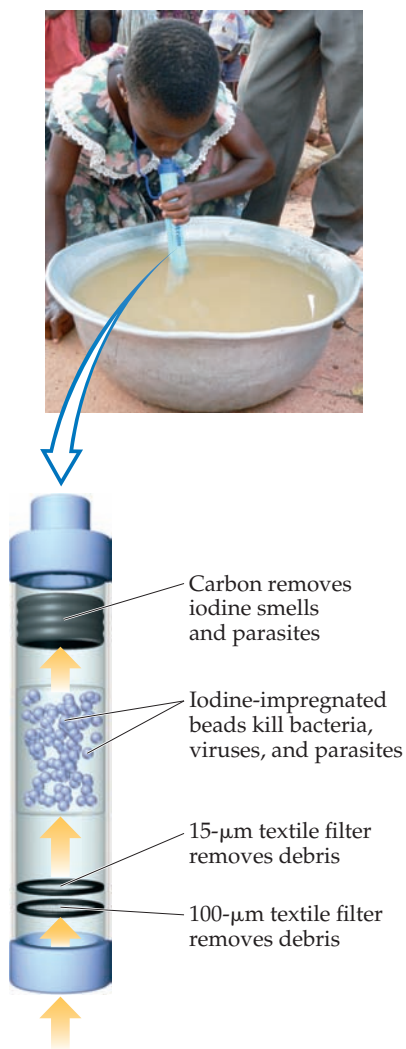
▲ Figure 18.21 A LifeStraw purifies water as it is drunk.
