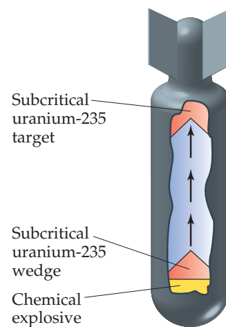
▲ Figure 21.16 Schematic drawing of an atomic bomb. A conventional explosive is used to bring two subcritical masses together to form a supercritical mass.
