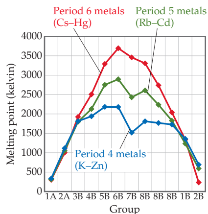
▲ Figure 12.21 The melting points of metals from periods 4, 5, and 6.
