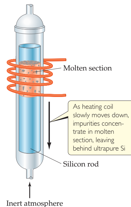
▲ Figure 22.32 Zone-refining apparatus for the production of ultrapure silicon.
