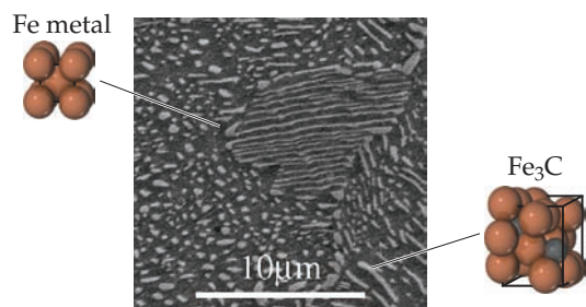
▲ Figure 12.16 Microscopic view of the structure of the heterogeneous alloy pearlite. The dark regions are body-centered cubic iron metal, and the lighter regions are cementite, \text{Fe}_3\text{C} .
