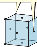
Face-centered cubic lattice
