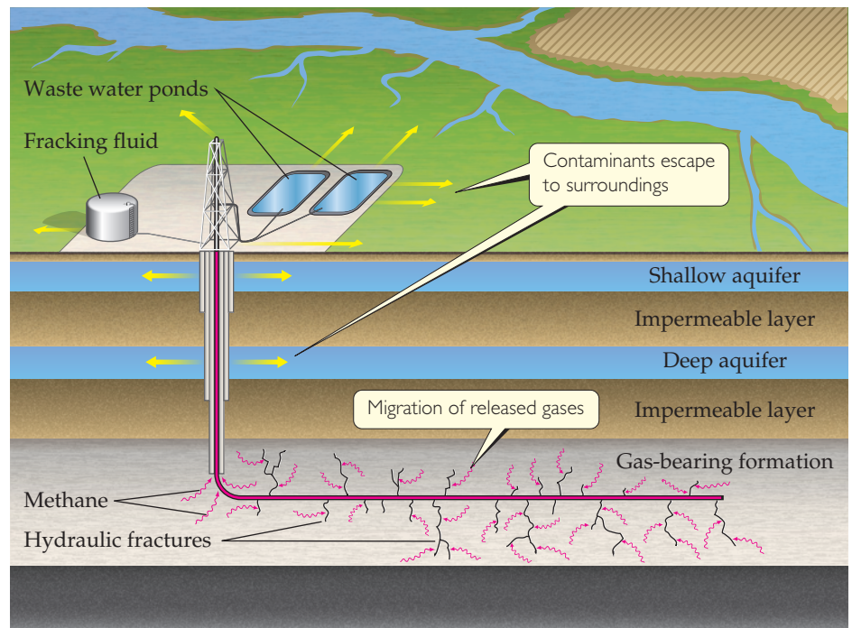
▲ Figure 18.22 A schematic of a well site employing fracking. The yellow arrows indicate the avenues through which contaminants enter the environment.
