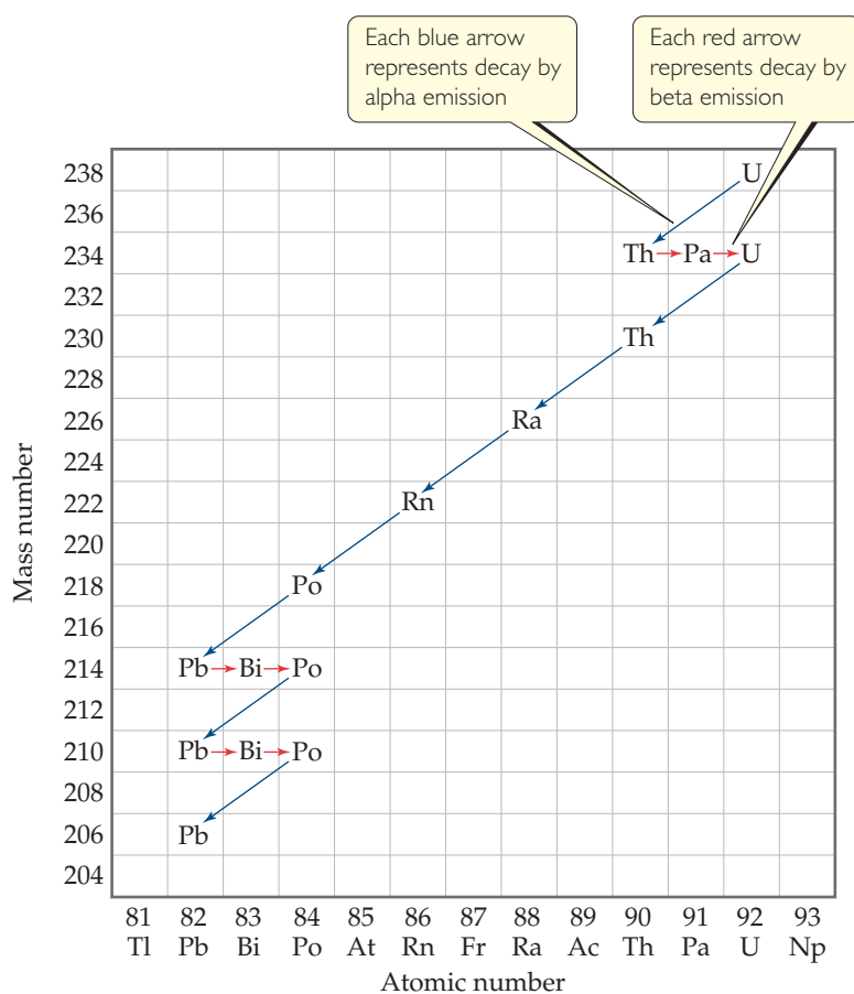
▲ Figure 21.3 Nuclear decay chain for uranium-238. The decay continues until the stable nucleus ^{206}\text{Pb} is formed.
