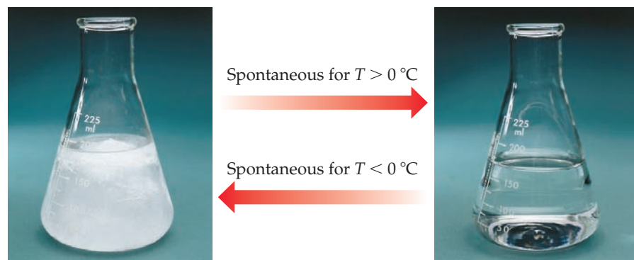
▲ Figure 19.3 Spontaneity can depend on temperature. At T > 0\text{ }^{\circ}\text{C} , ice melts spontaneously to liquid water. At T < 0\text{ }^{\circ}\text{C} , the reverse process, water freezing to ice, is spontaneous. At T = 0\text{ }^{\circ}\text{C} the two states are in equilibrium.
