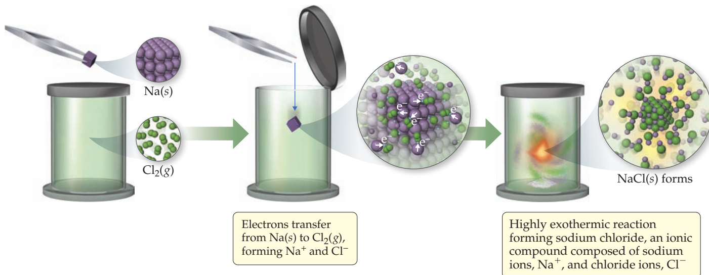
▲ Figure 8.2 Reaction of sodium metal with chlorine gas to form the ionic compound sodium chloride.
