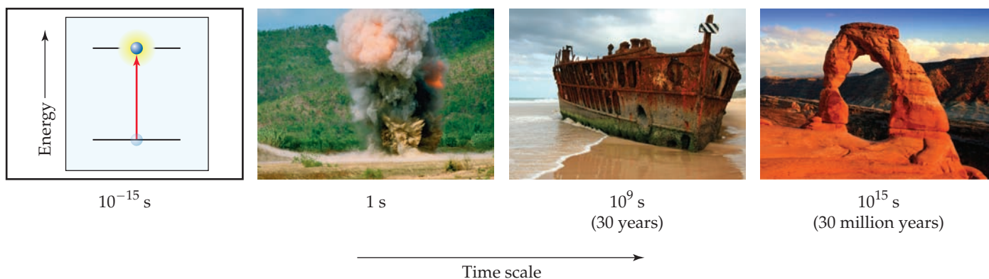
▲ Figure 14.1 Reaction rates span an enormous range of time scales. The absorption of light by an atom or a molecule is complete within one femtosecond; explosions occur within seconds; corrosion can occur over years; and the weathering of rocks can occur over millions of years.
