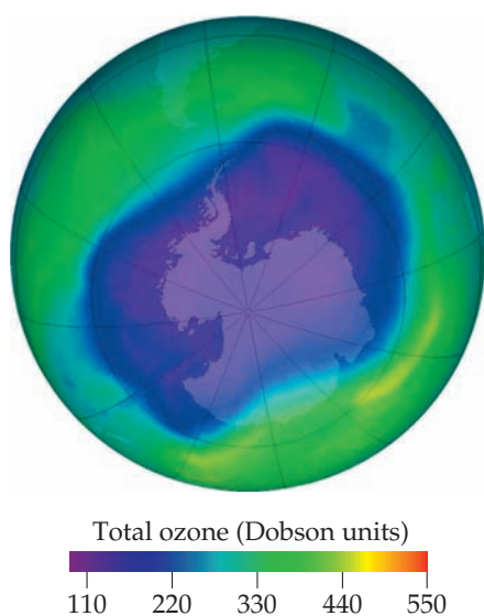
▲ Figure 18.6 Ozone present in the Southern Hemisphere, Sept. 24, 2006. The data were taken from an orbiting satellite. This day had the lowest stratospheric ozone concentration yet recorded. One “Dobson unit” corresponds to 2.69 \times 10^{16} ozone molecules in a 1 \text{ cm}^2 column of atmosphere.
