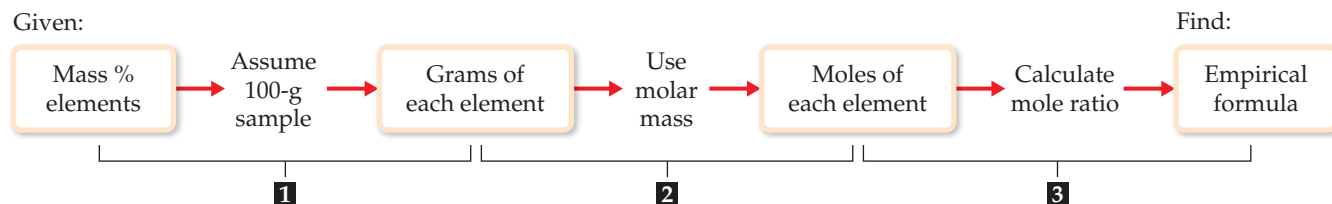
▲ Figure 3.13 Procedure for calculating an empirical formula from percentage composition.
