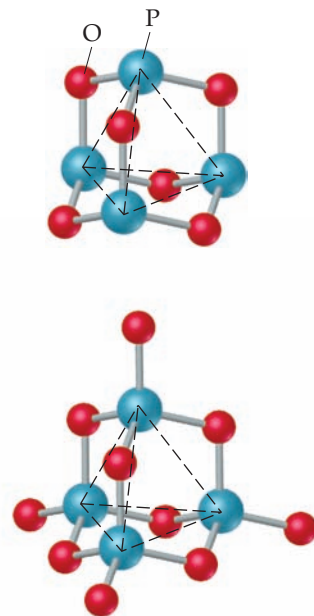
▲ Figure 22.27 Structures of \text{P}_4\text{O}_6 (top) and \text{P}_4\text{O}_{10} (bottom).
