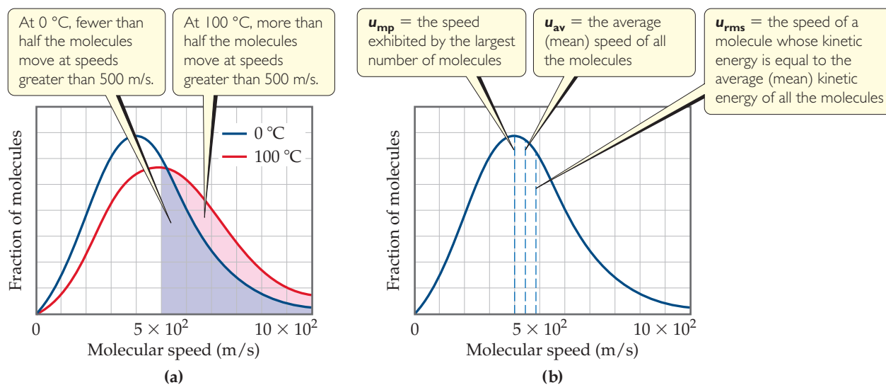
▲ Figure 10.13 Distribution of molecular speeds for nitrogen gas. (a) The effect of temperature on molecular speed. The relative area under the curve for a range of speeds gives the relative fraction of molecules that have those speeds. (b) Position of most probable ( u_{mp} ), average ( u_{av} ), and root-mean-square ( u_{rms} ) speeds of gas molecules. The data shown here are for nitrogen gas at 0 °C.
