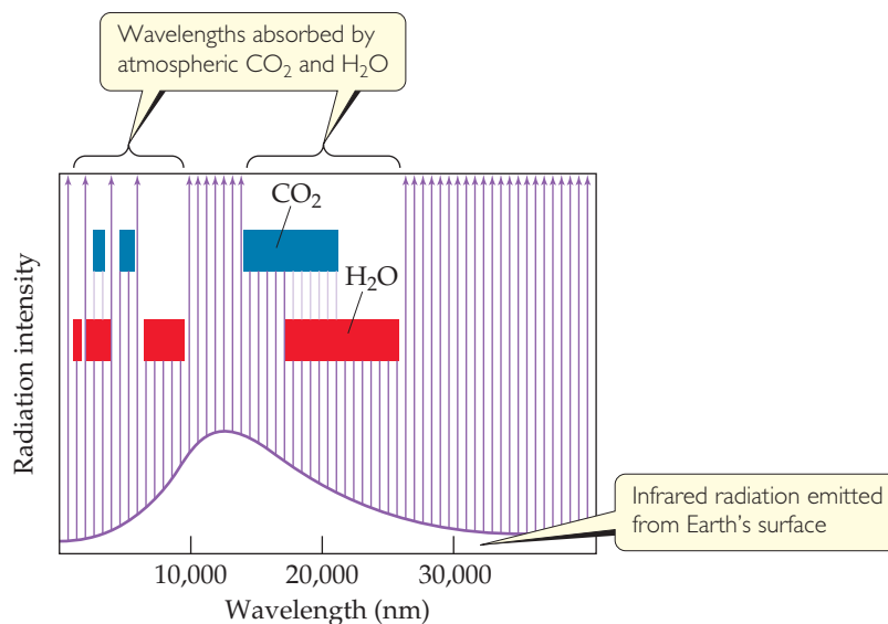
▲ Figure 18.12 Portions of the infrared radiation emitted by Earth's surface that are absorbed by atmospheric CO 2 and H 2 O.
