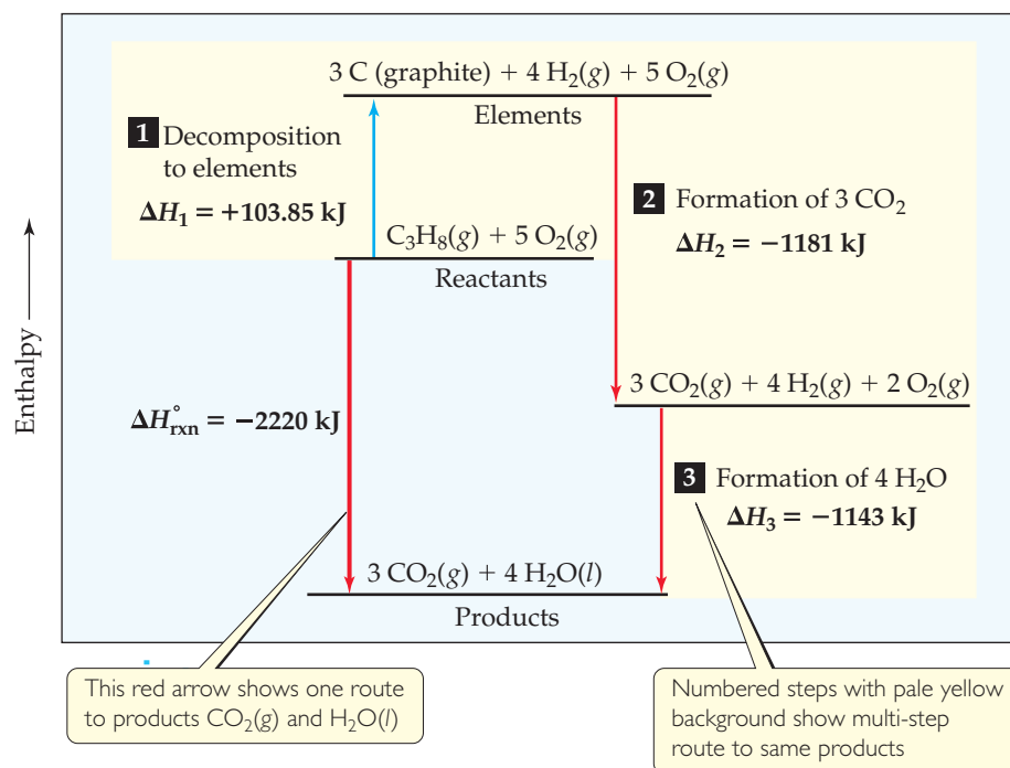
Figure 5.22 Enthalpy diagram for propane combustion.
