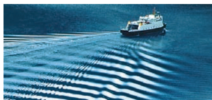
▲ Figure 6.1 Water waves. The movement of a boat through the water forms waves. The regular variation of peaks and troughs enables us to sense the motion of the waves away from the boat.
