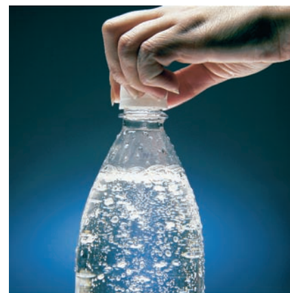
\blacktriangle Figure 13.14 Gas solubility decreases as pressure decreases. \text{CO}_2 bubbles out of solution when a carbonated beverage is opened because the \text{CO}_2 partial pressure above the solution is reduced.
