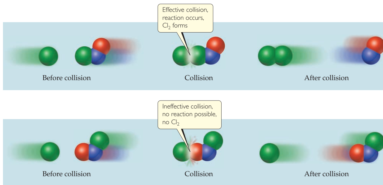
▲ Figure 14.15 Molecular collisions may or may not lead to a chemical reaction between Cl and NOCl .
