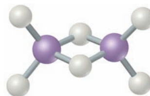
▲ Figure 22.35 The structure of diborane ( \text{B}_2\text{H}_6 ).
