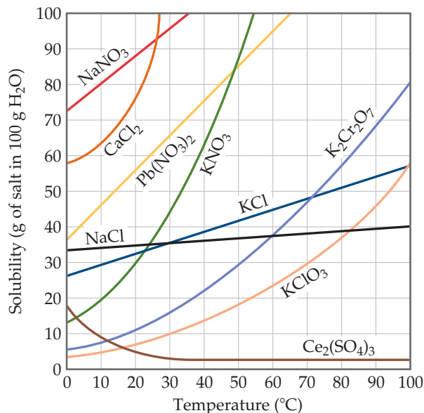
\blacktriangle Figure 13.15 Solubilities of some ionic compounds in water as a function of temperature.
