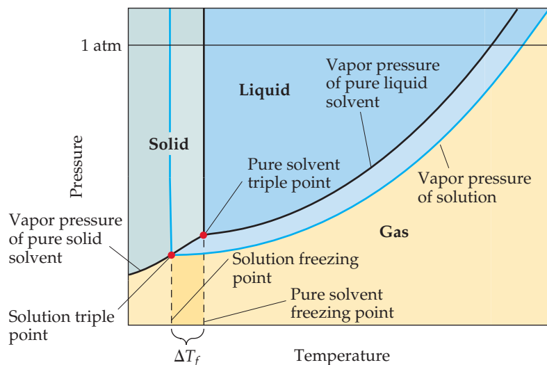
▲ Figure 13.21 Phase diagram illustrating freezing-point depression. The black lines show the pure solvent's phase equilibria curves, and the blue lines show the solution's phase equilibria curves.
