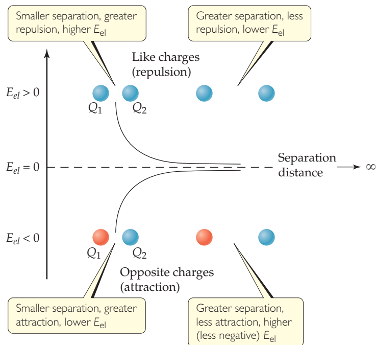
▲ Figure 5.3 Electrostatic potential energy. At finite separation distances for two charged particles, E_{el} is positive for like charges and negative for opposite charges. As the particles move farther apart, their electrostatic potential energy approaches zero.
