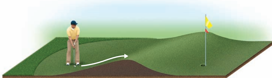
▲ Figure 14.16 Energy is needed to overcome a barrier between initial and final states.
