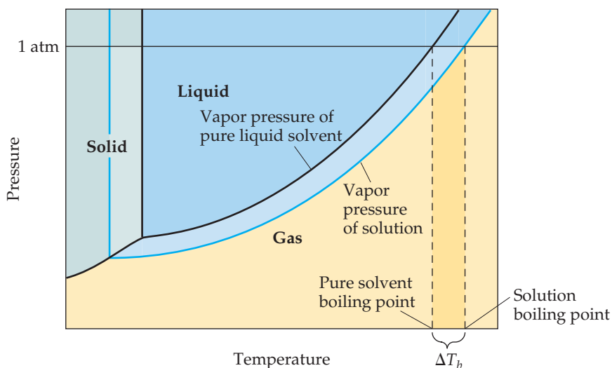
▲ Figure 13.20 Phase diagram illustrating boiling-point elevation. The black lines show the pure solvent's phase equilibria curves, and the blue lines show the solution's phase equilibria curves.
