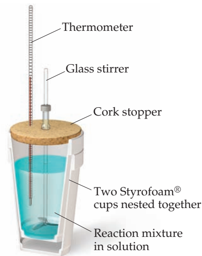
▲ Figure 5.17 Coffee-cup calorimeter. This simple apparatus is used to measure temperature changes of reactions at constant pressure.
