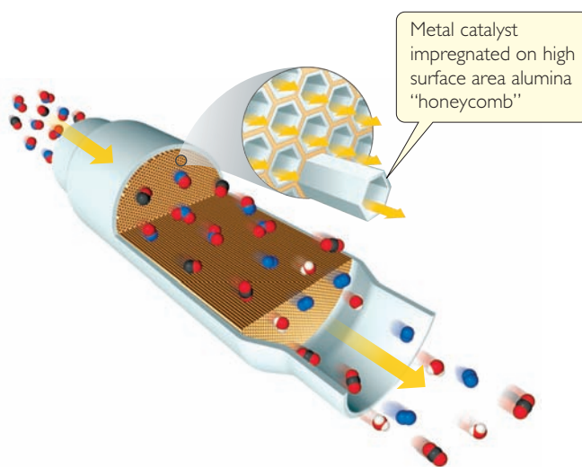
▲ Figure 14.25 Cross section of a catalytic converter.
