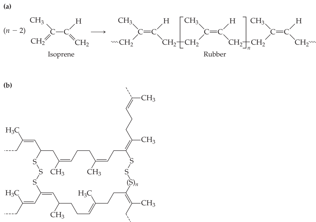
▲ Figure 12.41 Vulcanization of natural rubber. (a) Formation of polymeric natural rubber from the monomer isoprene. (b) Adding sulfur to rubber creates carbon–sulfur bonds, and sulfur–atom links between chains.
