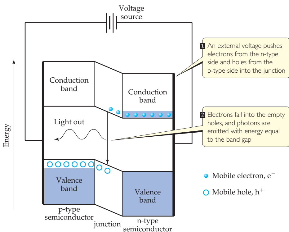
▲ Figure 12.32 Light-emitting diodes. The heart of a light-emitting diode is a p-n junction in which an applied voltage drives electrons and holes together, where they combine and give off light.
