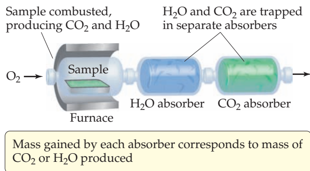
▲ Figure 3.14 Apparatus for combustion analysis.
