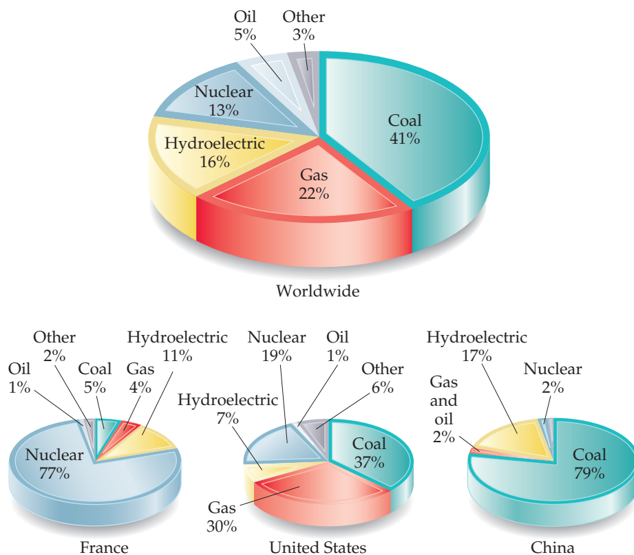
▲ Figure 21.1 Sources of electricity generation, worldwide and for select countries (Sources: U.S. Energy Information Administration and the International Energy Agency, 2010–2012 data).
