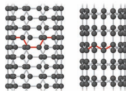
▲ Figure 12.48 Atomic models of carbon nanotubes. Left: “Armchair” nanotube, which shows metallic behavior. Right: “Zigzag” nanotube, which can be either semiconducting or metallic, depending on tube diameter.
