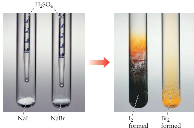
▲ Figure 22.10 Reaction of \text{H}_2\text{SO}_4 with \text{NaI} and \text{NaBr} .
