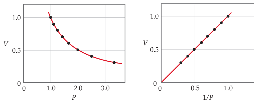
▲ Figure 10.6 Boyle's Law. For a fixed quantity of gas at constant temperature, the volume of the gas is inversely proportional to its pressure.
