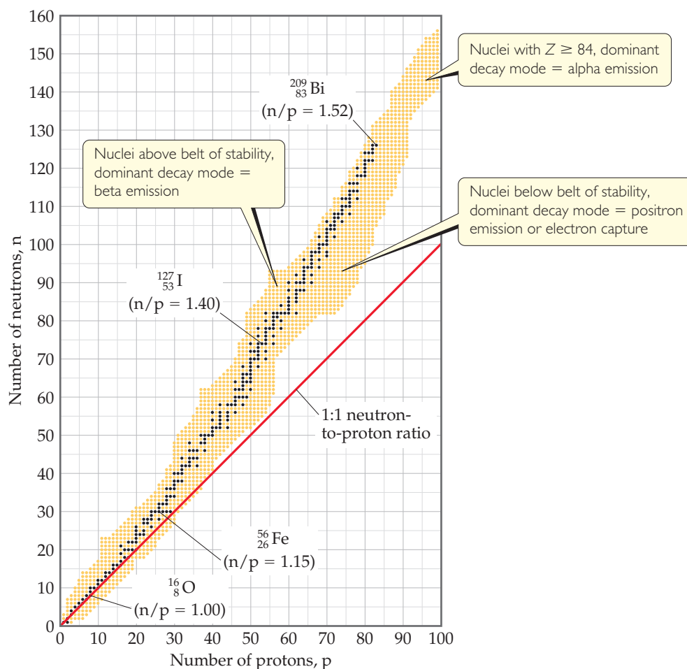
▲ Figure 21.2 Stable and radioactive isotopes as a function of numbers of neutrons and protons in a nucleus. The stable nuclei (dark blue dots) define a region known as the belt of stability.
