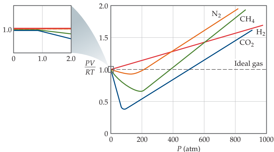
▲ Figure 10.19 The effect of pressure on the behavior of several real gases. Data for 1 mol of gas in all cases. Data for N_2 , CH_4 , and H_2 are at 300 K; for CO_2 data are at 313 K because under high pressure CO_2 liquefies at 300 K.
