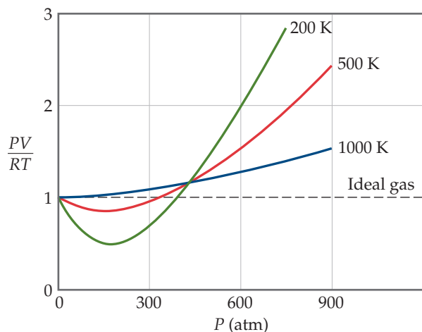
▲ Figure 10.20 The effect of temperature and pressure on the behavior of nitrogen gas.
