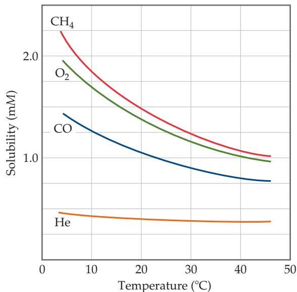
\blacktriangle Figure 13.16 Solubilities of four gases in water as a function of temperature. The solubilities are in millimoles per liter of solution, for a constant total pressure of 1 atm in the gas phase.
