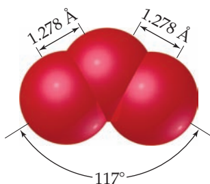
▲ Figure 8.12 Molecular structure of ozone.
