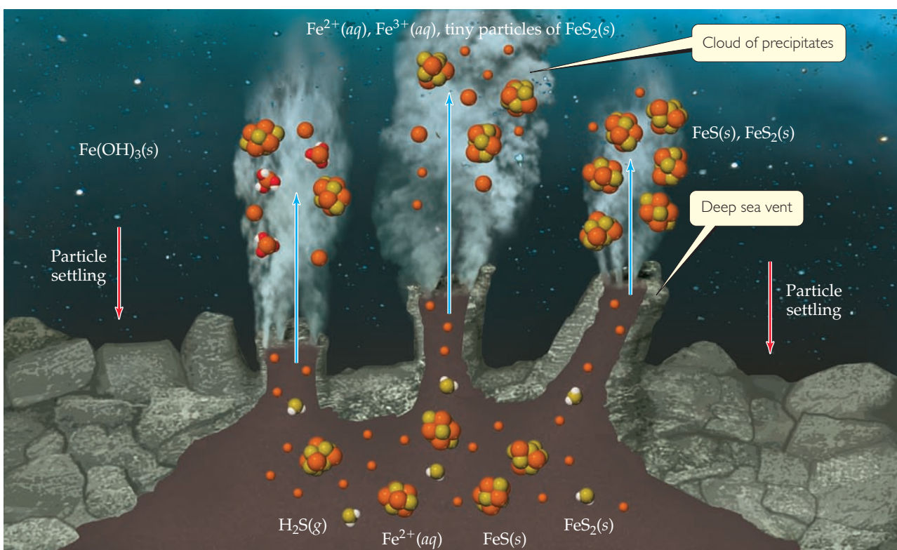
▲ Figure 4.1 Researchers have recently found that compounds containing iron, sulfur, and oxygen are the reactants and products in a deep sea vent.
