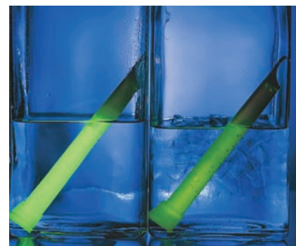
▲ Figure 14.13 Temperature affects the rate of the chemiluminescence reaction in light sticks: The chemiluminescent reaction occurs more rapidly in hot water, and more light is produced.
