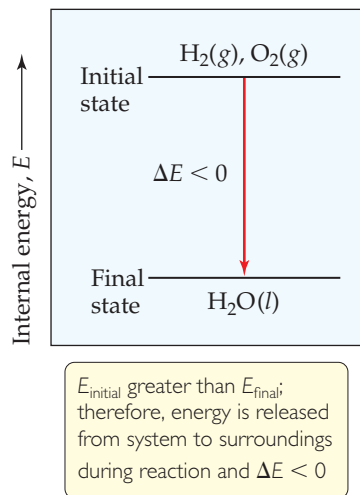
▲ Figure 5.6 Energy diagram for the reaction 2 \text{H}_2(g) + \text{O}_2(g) \longrightarrow 2 \text{H}_2\text{O}(l) .
