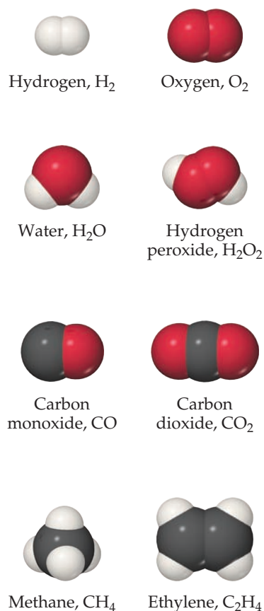
▲ Figure 2.16 Molecular models. Notice how the chemical formulas of these simple molecules correspond to their compositions.
