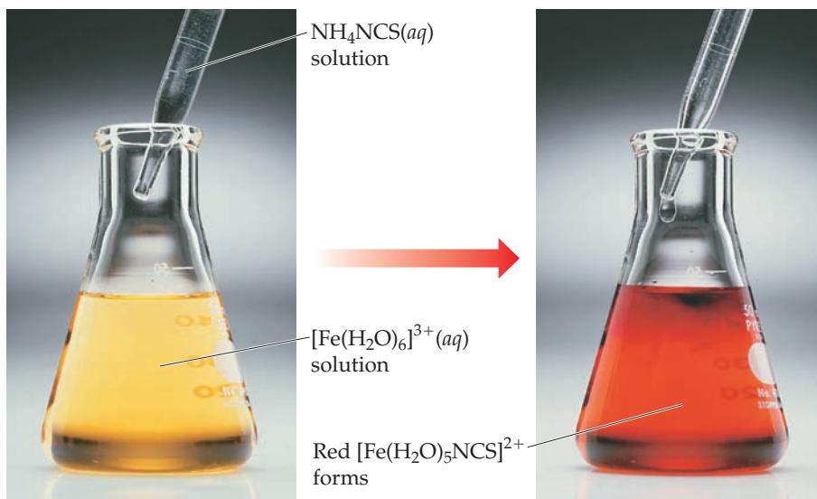
▲ Figure 23.9 Reaction of \text{Fe}^{3+}(aq) and \text{NCS}^-(aq) .
