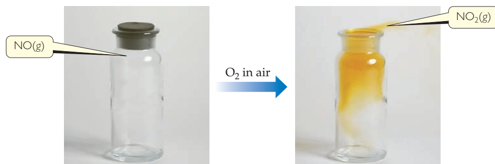
▲ Figure 22.24 Formation of \text{NO}_2(g) as \text{NO}(g) combines with \text{O}_2(g) in the air.
