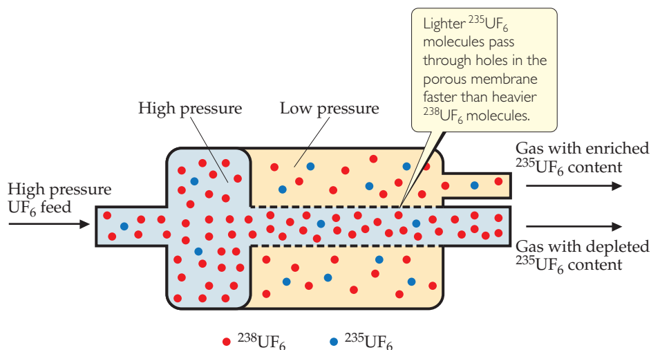
▲ Figure 10.17 Uranium enrichment by gaseous diffusion. The lighter ^{235}\text{UF}_6 effuses through a porous barrier at a slightly faster rate than ^{238}\text{UF}_6 . The pressure difference across the membrane drives the effusion. The enrichment shown here for a single step is exaggerated for illustrative purposes.
