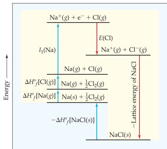
▲ Figure 8.5 Born-Haber cycle for formation of \text{NaCl} . This Hess's law representation shows the energetic relationships in the formation of the ionic solid from its elements.
