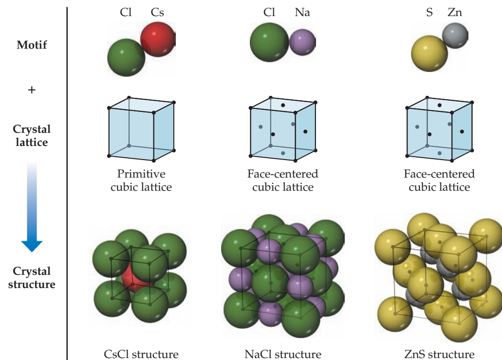
▲ Figure 12.25 The structures of CsCl, NaCl, and ZnS. Each structure type can be generated by the combination of a two-atom motif and the appropriate lattice.
