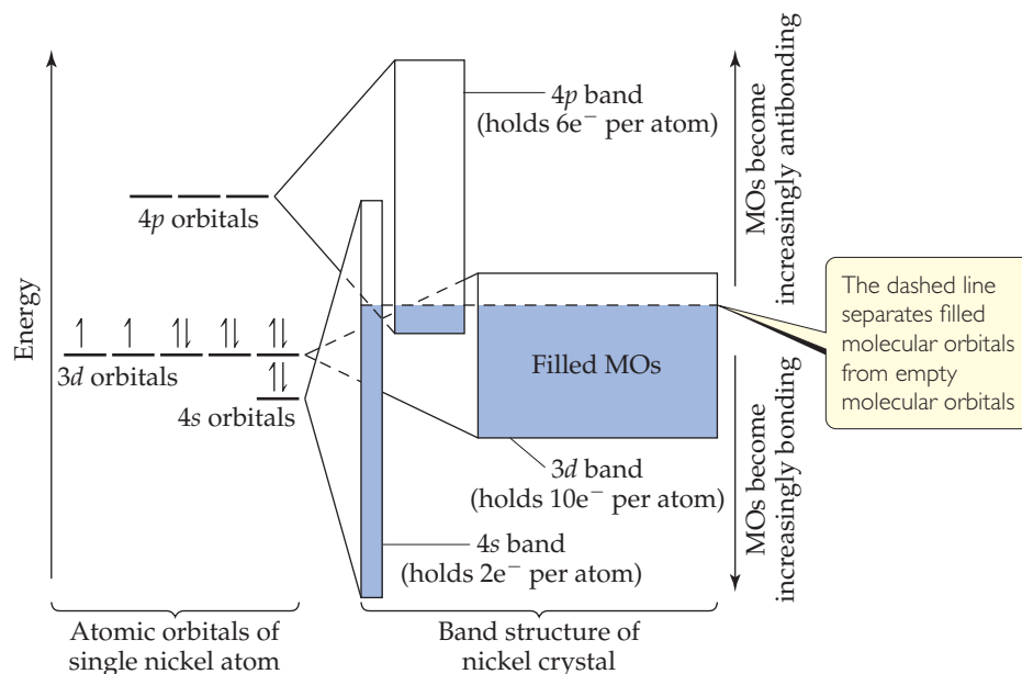
▲ Figure 12.23 The electronic band structure of nickel.
