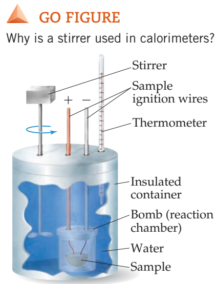
▲ Figure 5.18 Bomb calorimeter.
