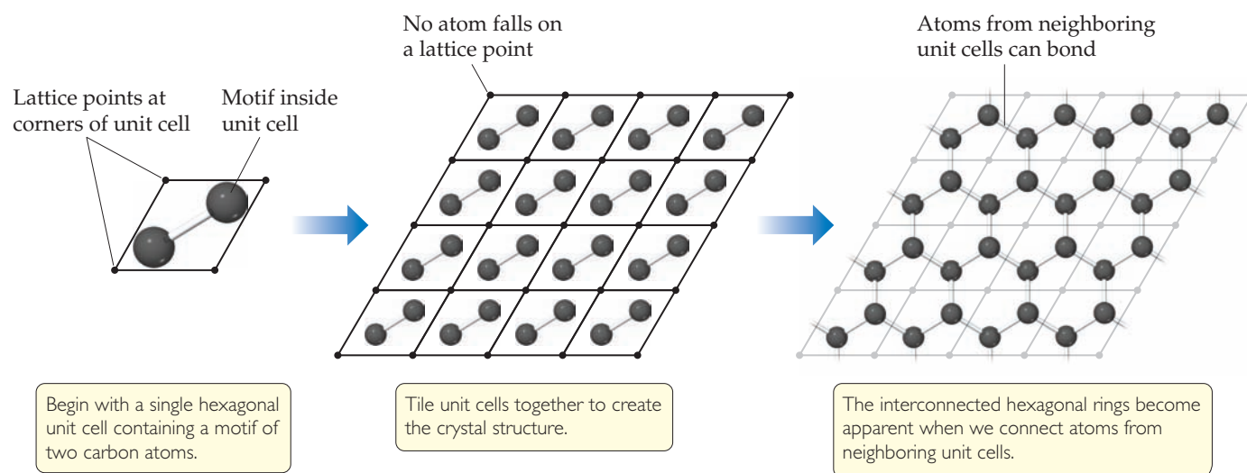
▲ Figure 12.8 Two-dimensional structure of graphene built up from a single unit cell.
