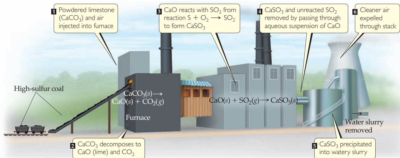
▲ Figure 18.9 One method for removing \text{SO}_2 from combusted fuel.
