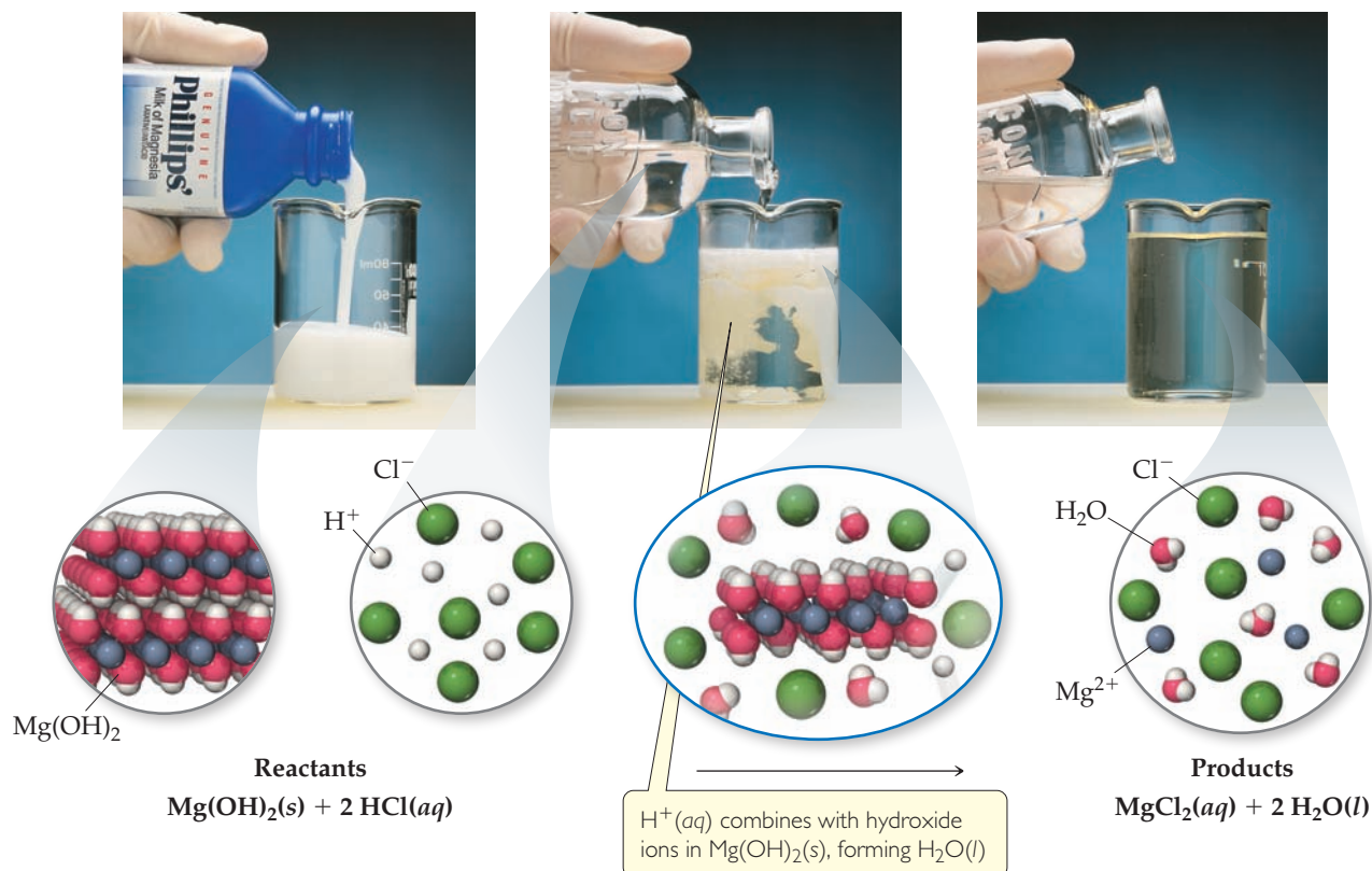
▲ Figure 4.9 Neutralization reaction between \text{Mg}(\text{OH})_2(s) and hydrochloric acid. Milk of magnesia is a suspension of water-insoluble magnesium hydroxide, \text{Mg}(\text{OH})_2(s) , in water. When sufficient hydrochloric acid, \text{HCl}(aq) , is added, a reaction ensues that leads to an aqueous solution containing \text{Mg}^{2+}(aq) and \text{Cl}^{-}(aq) ions.
