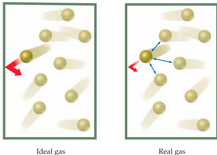
▲ Figure 10.22 In any real gas, attractive intermolecular forces reduce pressure to values lower than in an ideal gas.
