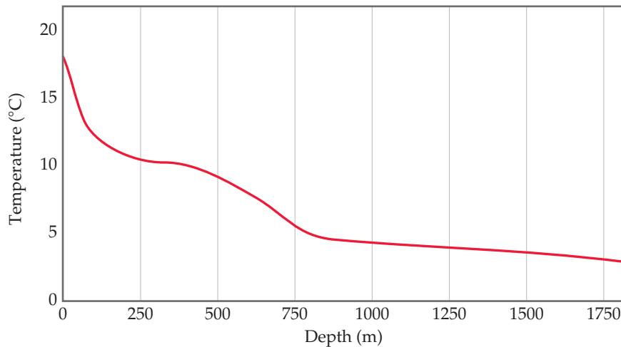
▲ Figure 18.16 Typical average temperature of mid-latitude seawater as a function of depth.
