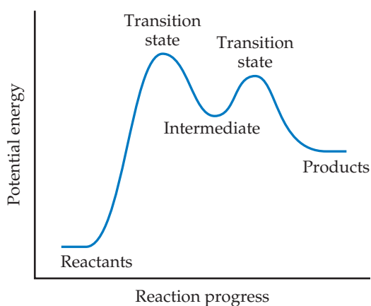
▲ Figure 14.20 The energy profile of a reaction, showing transition states and an intermediate.
