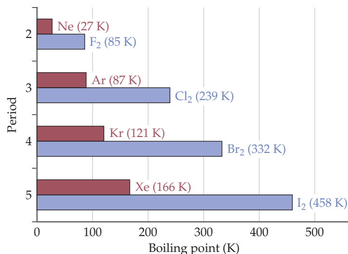
▲ Figure 11.5 Boiling points of the halogens and noble gases. This plot shows how the boiling points increase due to stronger dispersion forces as the molecular weight increases.
