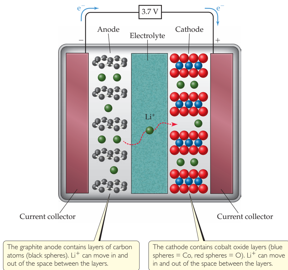
▲ Figure 20.21 Schematic of a Li-ion battery. When the battery is discharging (operating) \text{Li}^+ ions move out of the anode and migrate through the electrolyte where they enter the spaces between the cobalt oxide layers, reducing the cobalt ions. To recharge the battery, electrical energy is used to drive the \text{Li}^+ back to the anode, oxidizing the cobalt ions in the cathode.
